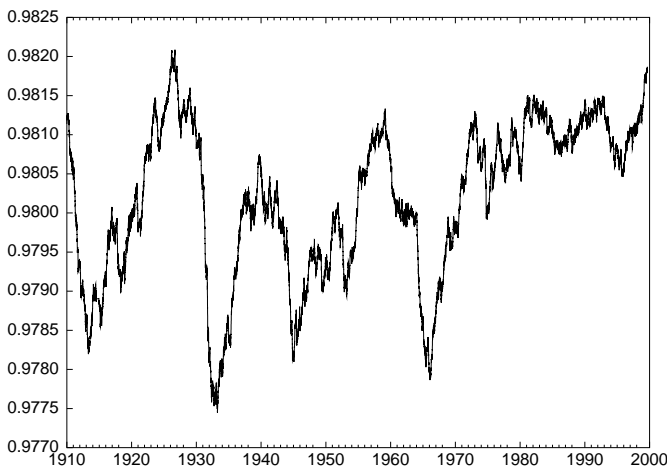
Fig. 4. Moving exponential average of the local uncertainty h_5 with an halflife period of 5 years for the full dataset.
