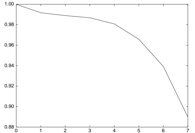
Fig. 2. Conditional entropy h_n = H_{n+1} - H_n as a function of word length n . Beyond n = 5 the calculation of the conditional entropy is not reliable due to large statistical errors [8, 9].
